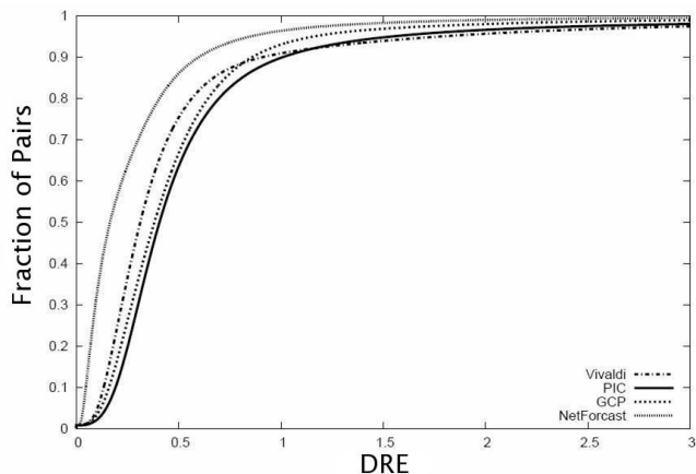
Fig. 1. DRE distribution
