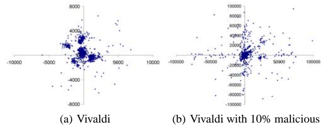
Figure 1: Effect of Disorder attack with 1740 nodes
