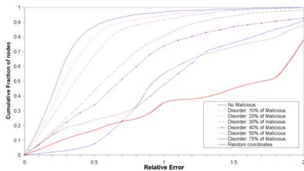
Figure 3: Genesis disorder attack: CDF of relative error at simulation tick = 2000
