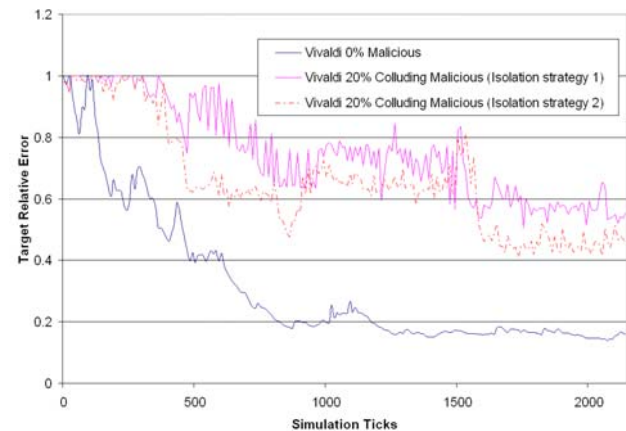
Figure 14: Colluding Isolation attack 2: target relative error
