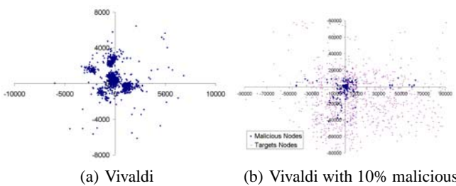
Figure 7: Effect of Repulsion attack with 1740 nodes
