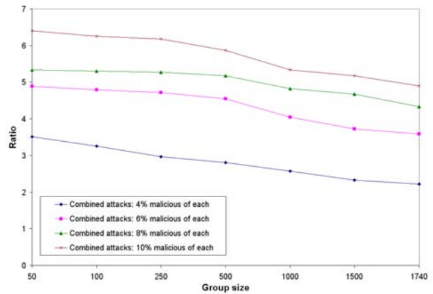
Figure 17: Combined attacks: effect of system size.
