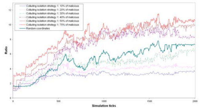
Figure 13: Genesis Colluding isolation Attack: average relative error ratio
