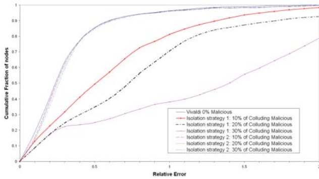
Figure 15: Colluding Isolation Attack: CDF of relative errors.
