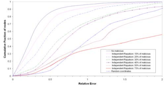
Figure 8: CDF of relative error.
