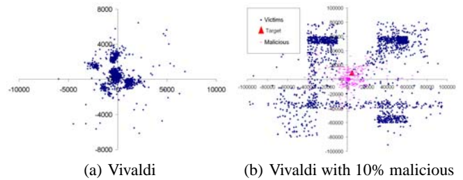
Figure 12: Effect of Colluding Isolation attack with 1740 nodes
