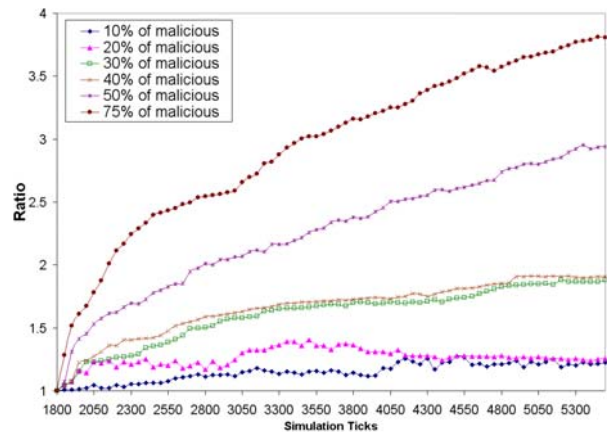
Figure 5: Injection of Disorder Attackers: average relative error ratio.
