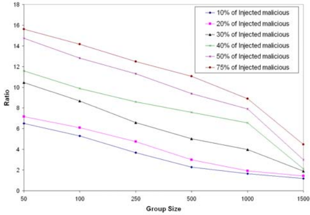
Figure 6: Injection of Disorder Attackers: Impact of system size on the attack.
