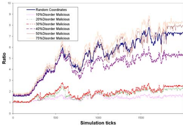
Figure 2: Genesis Disorder Attack: Variation of the ratio of average relative error in presence of malicious nodes.
