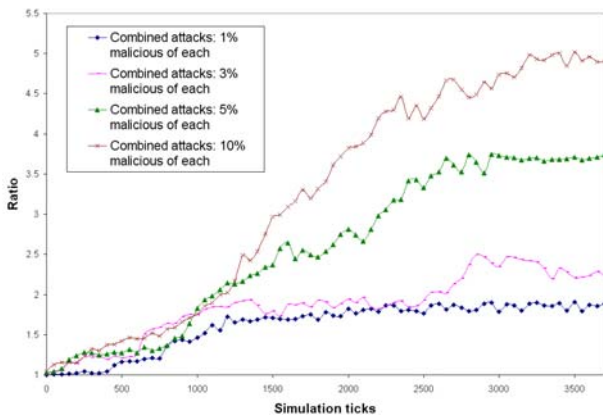
Figure 16: Combining attacks: impact on convergence.
