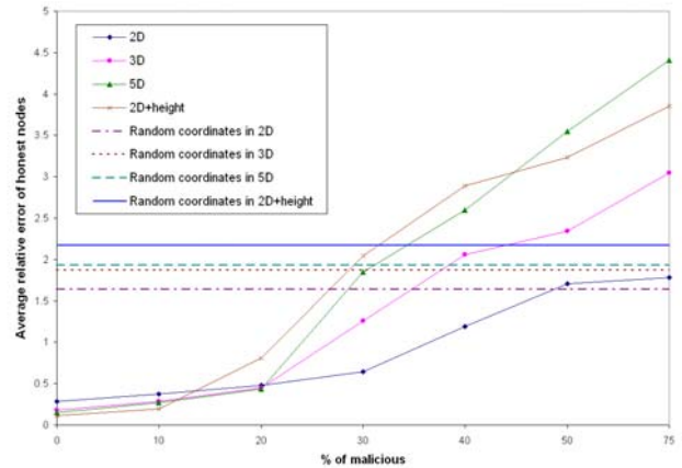
Figure 4: Genesis Disorder Attack: Impact of space dimensions
