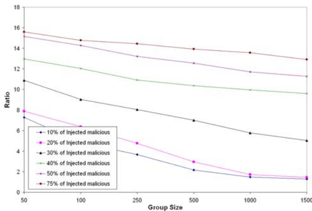
Figure 11: Injection Repulsion Attack: effect of system size
