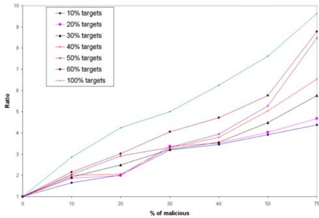
Figure 10: Genesis Repulsion Attack on subsets of target nodes.
