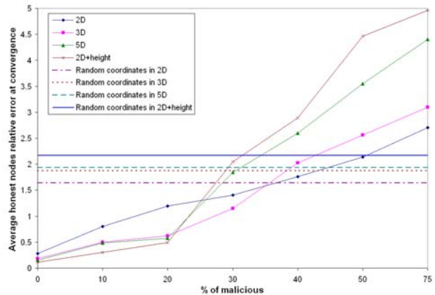
Figure 9: Genesis Repulsion Attack: impact of space dimensions.
